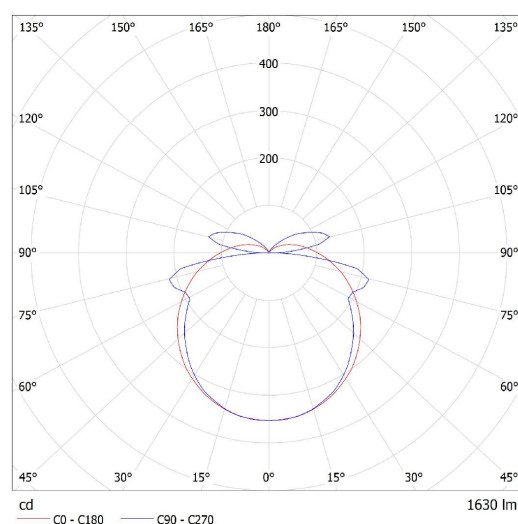
Lucis S1.L12 W PA MAIA PMMA LED / LDC (Polar)
